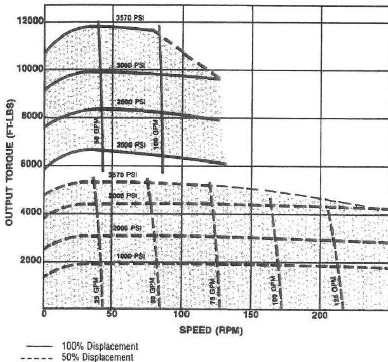
MRH2-270 Performance Curve
