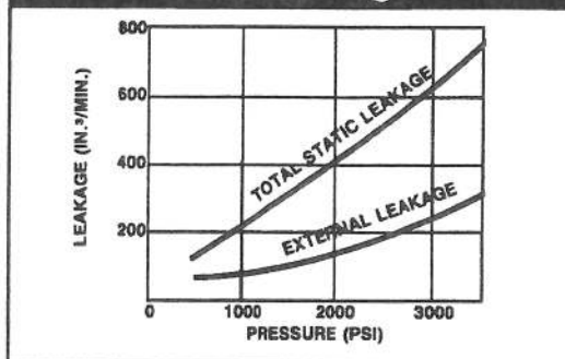
Static Leakage
