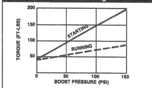
Torque Requirement When Free Wheeling
