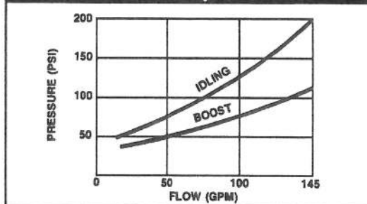
Idling Pressure and Boost Pressure Requirement
